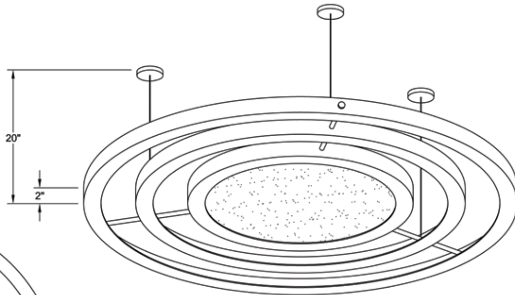
ISOMETRIC
