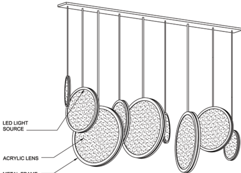
ISOMETRIC
