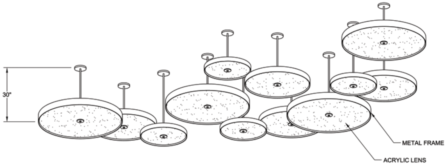
ISOMETRIC
