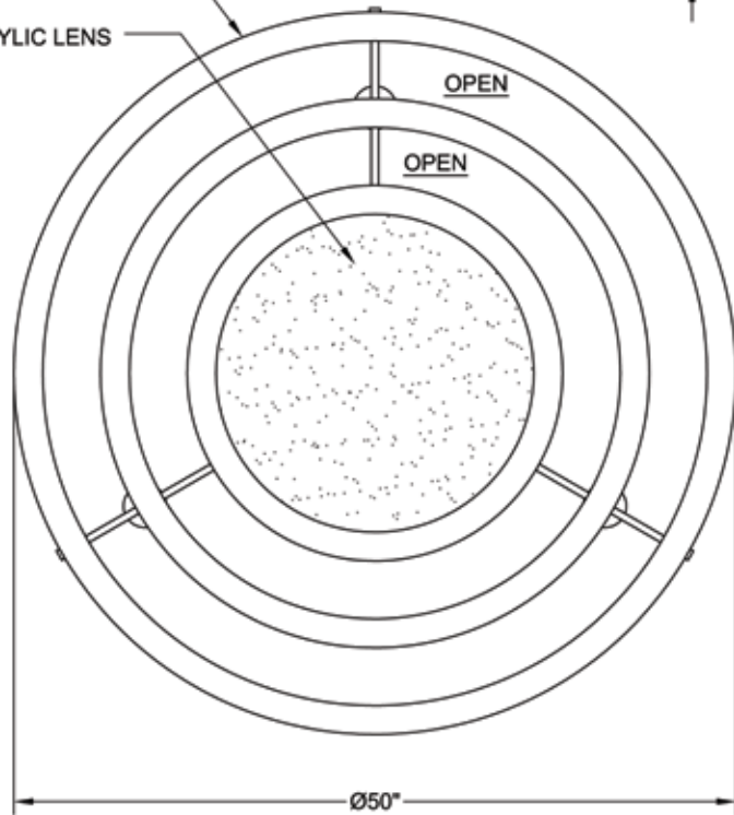
PLAN VIEW
